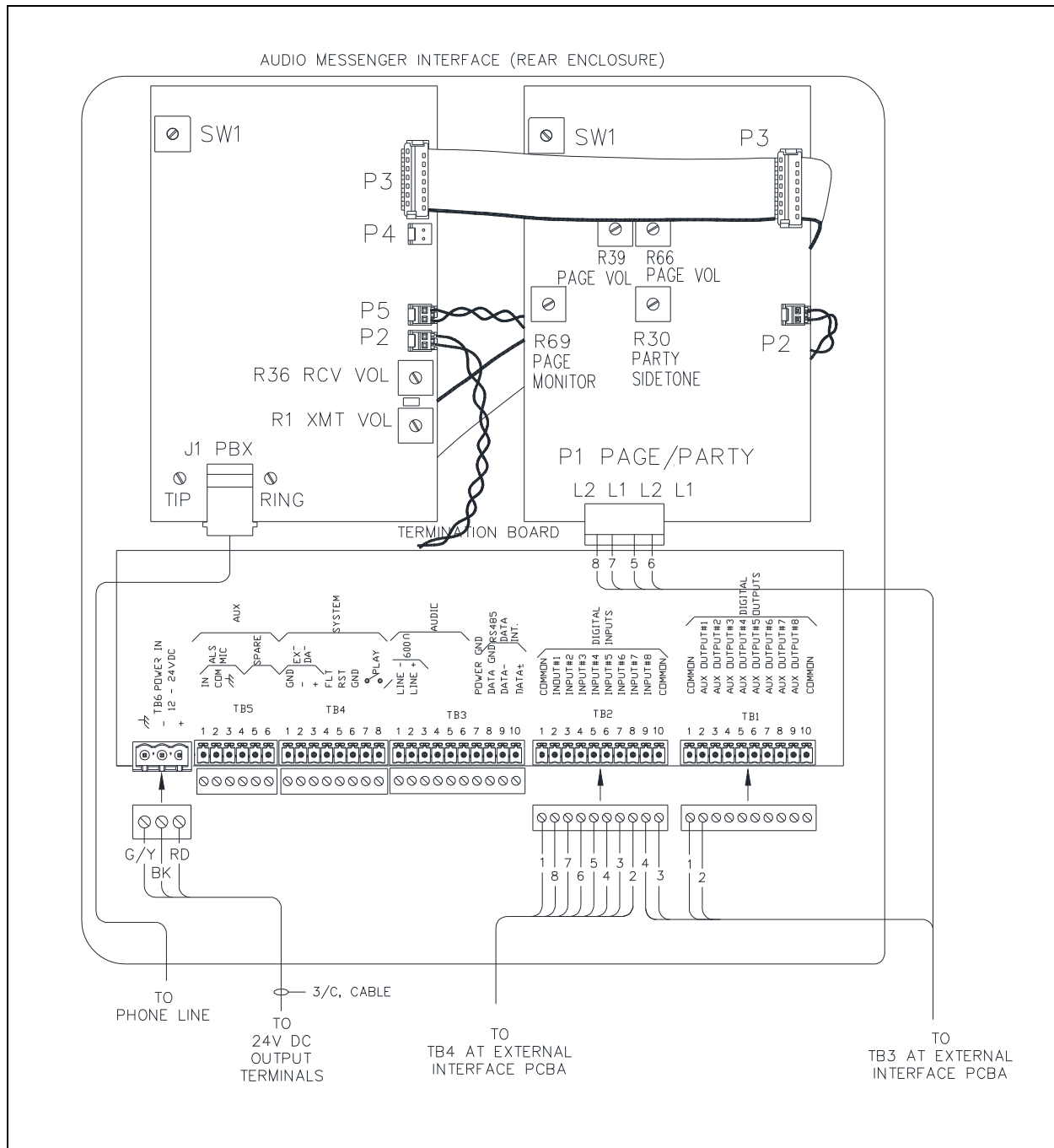
Figure 4. Audio Messenger Interface Connection Diagram
